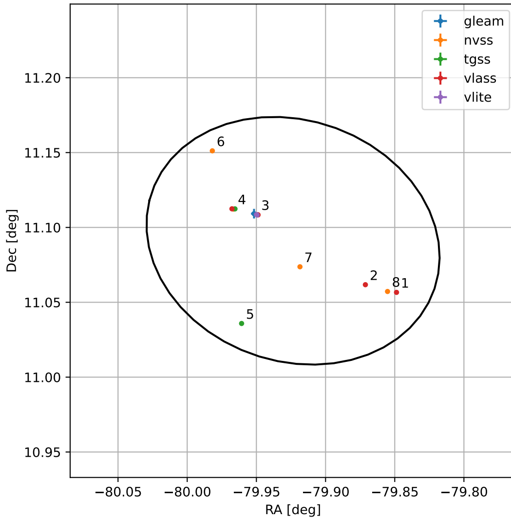
4FGL J1840.3+1105
