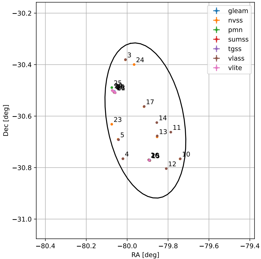
4FGL J1840.3-3037
