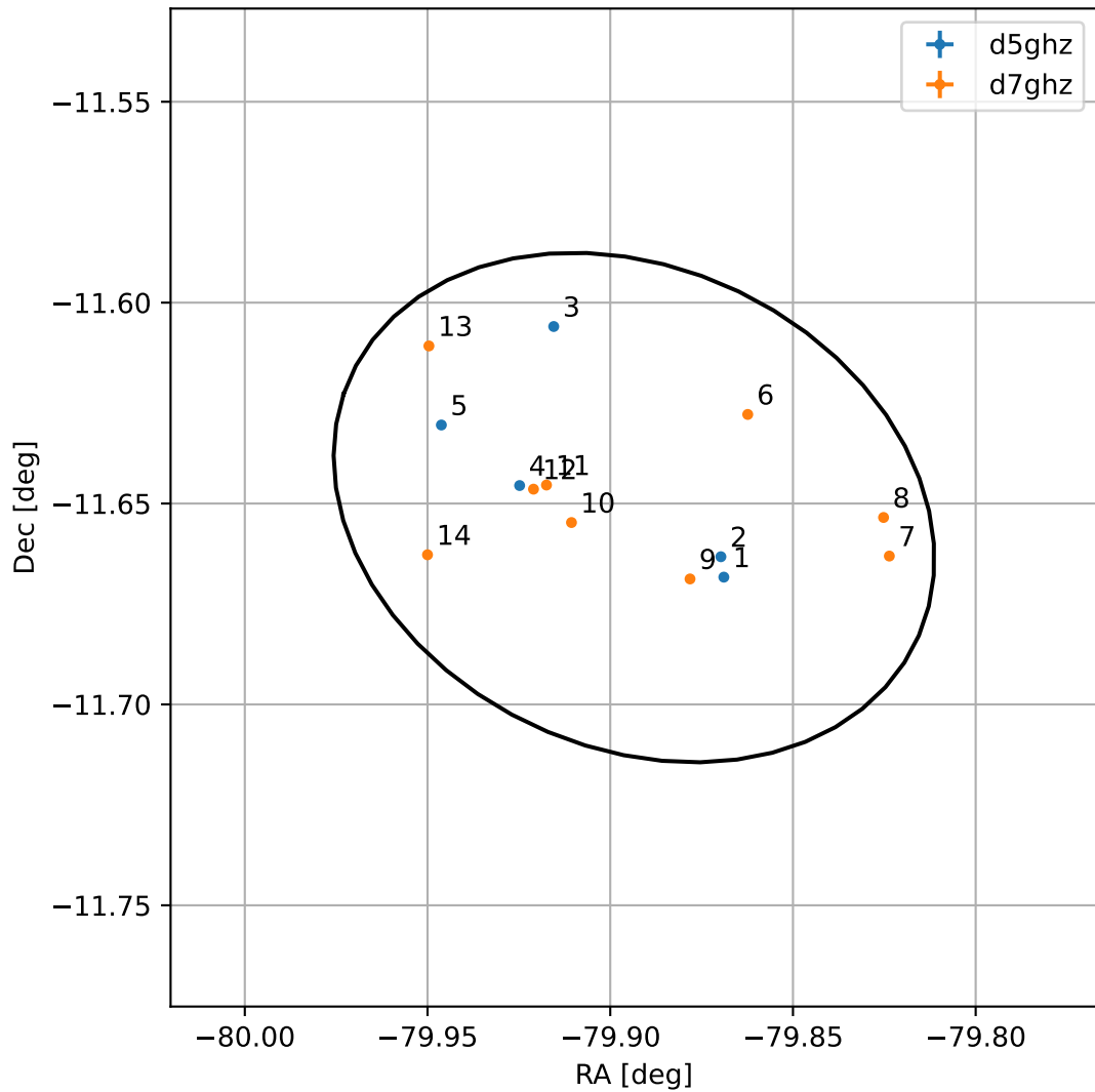
4FGL J1840.4-1139
