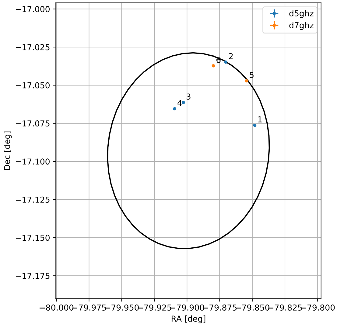
4FGL J1840.4-1705
