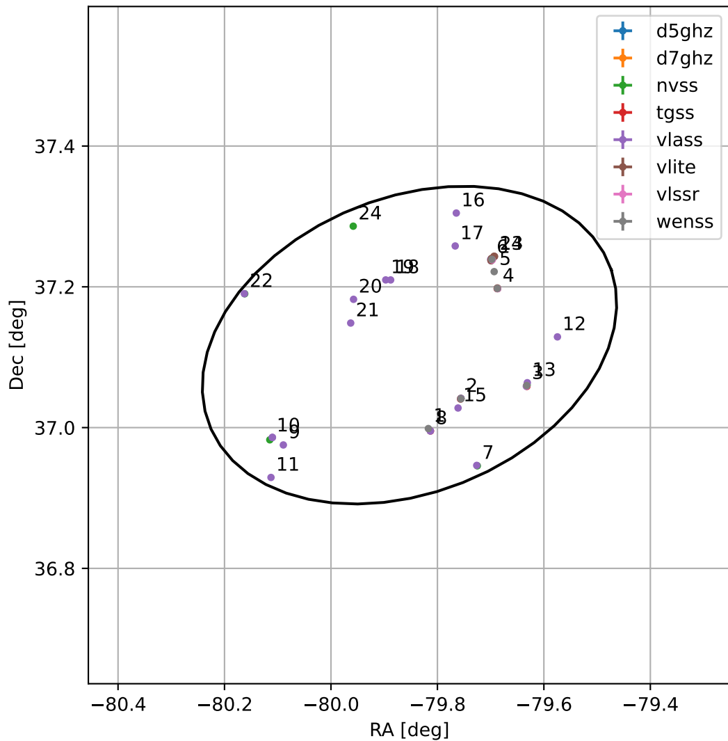
4FGL J1840.5+3707
