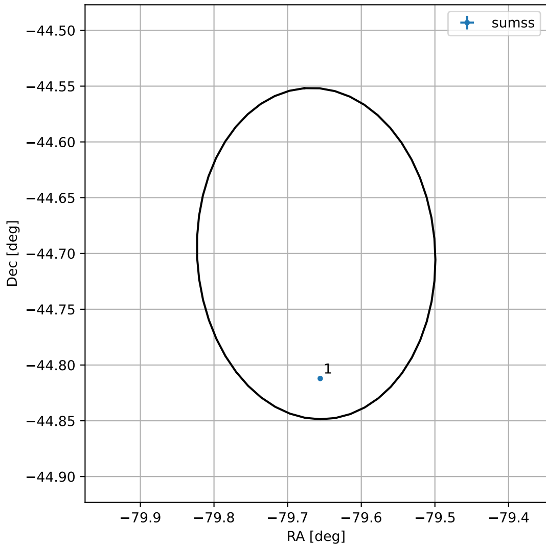
4FGL J1841.3-4442
