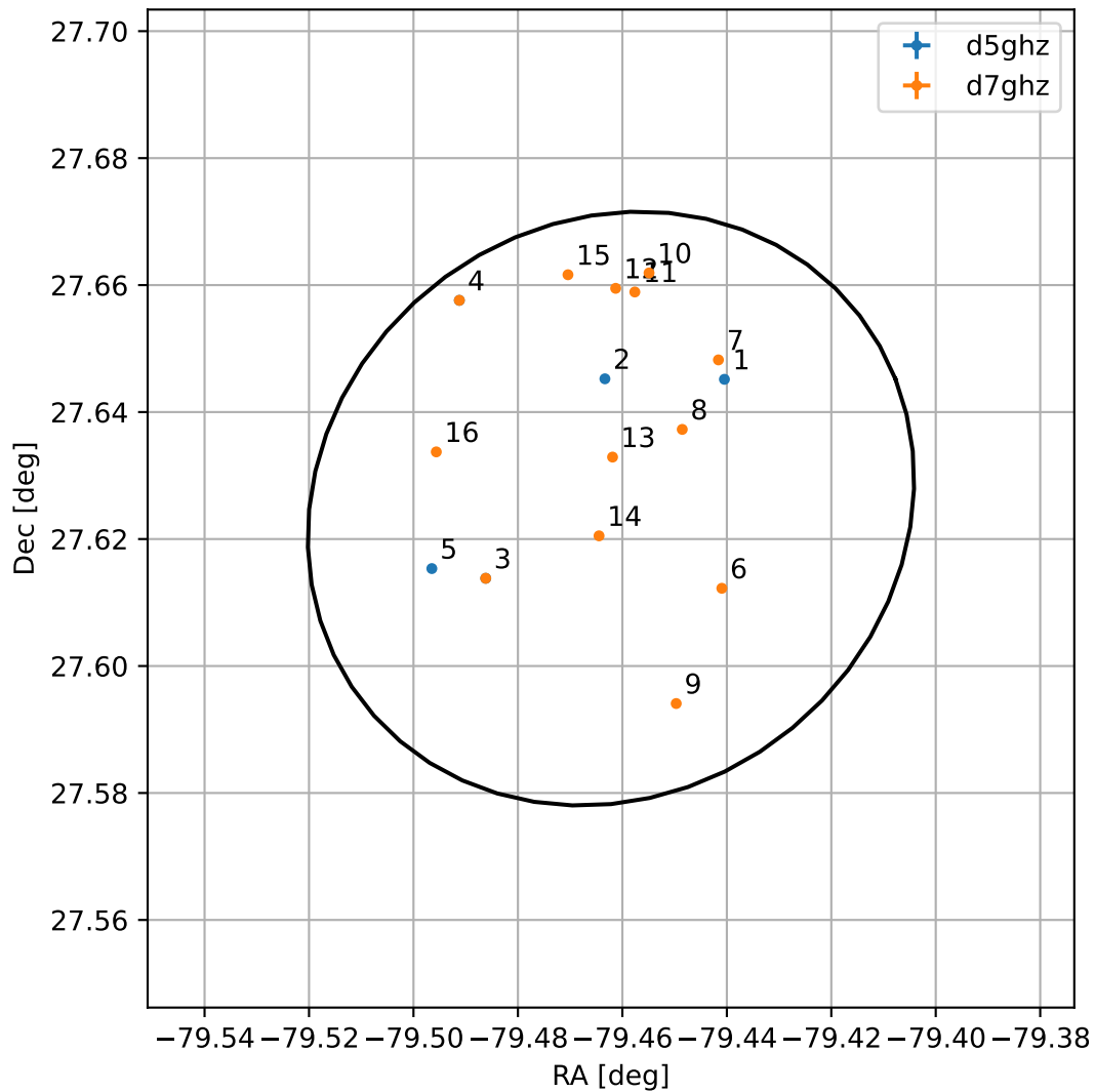
4FGL J1842.1+2737
