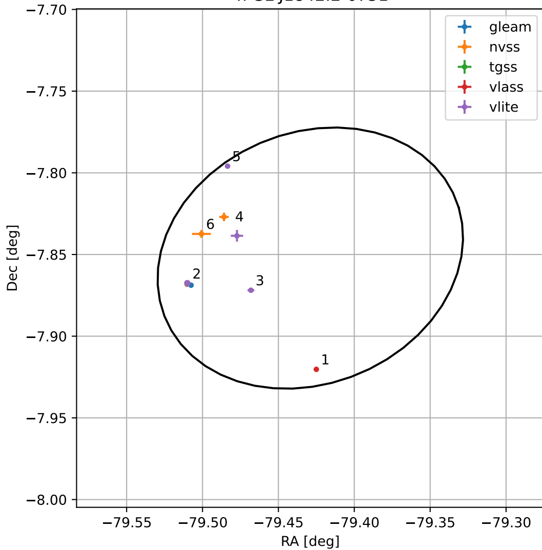
4FGL J1842.2-0751
