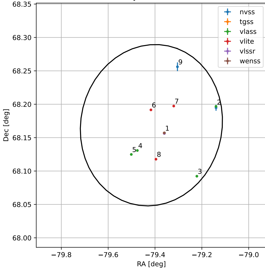
4FGL J1842.3+6810
