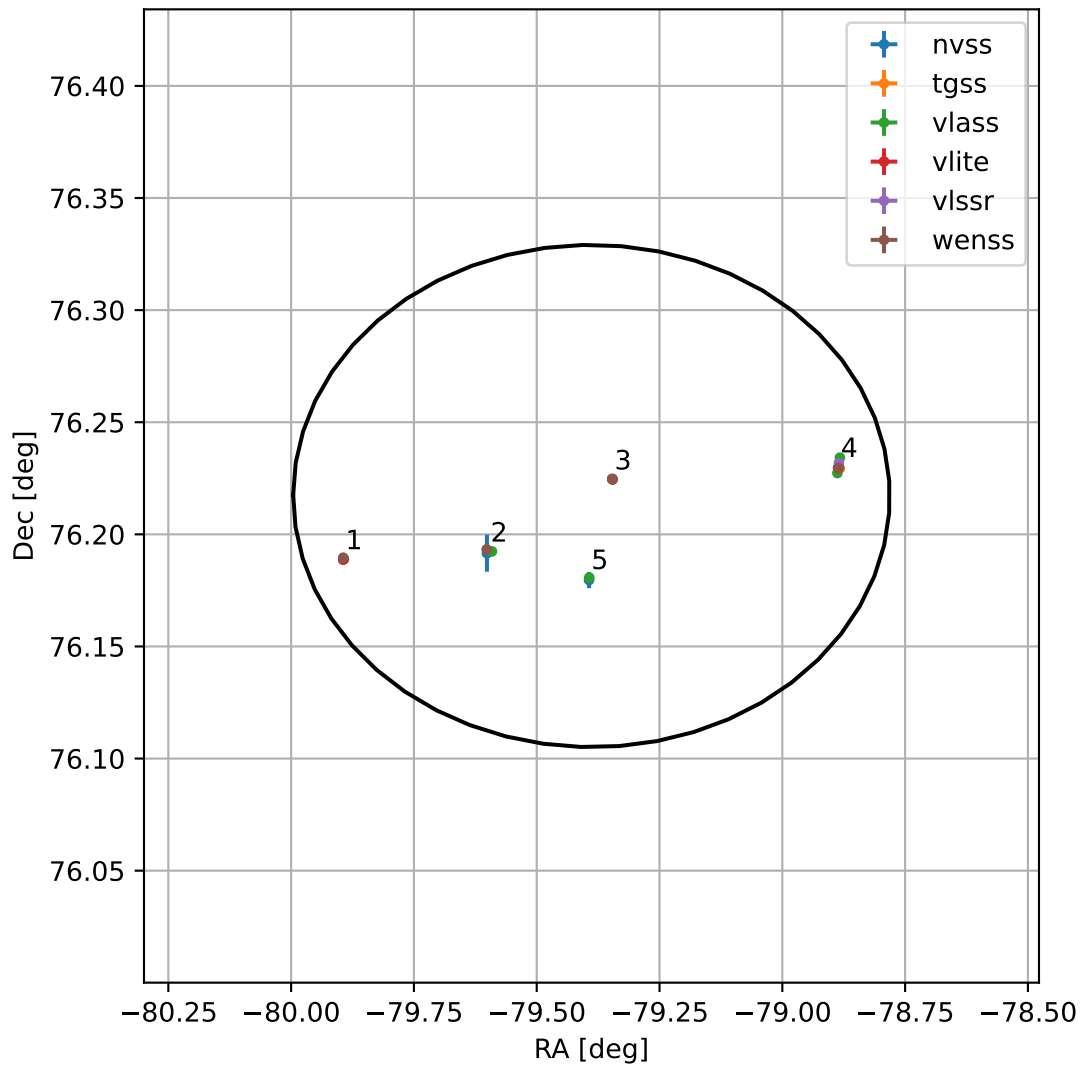
4FGL J1842.4+7613
