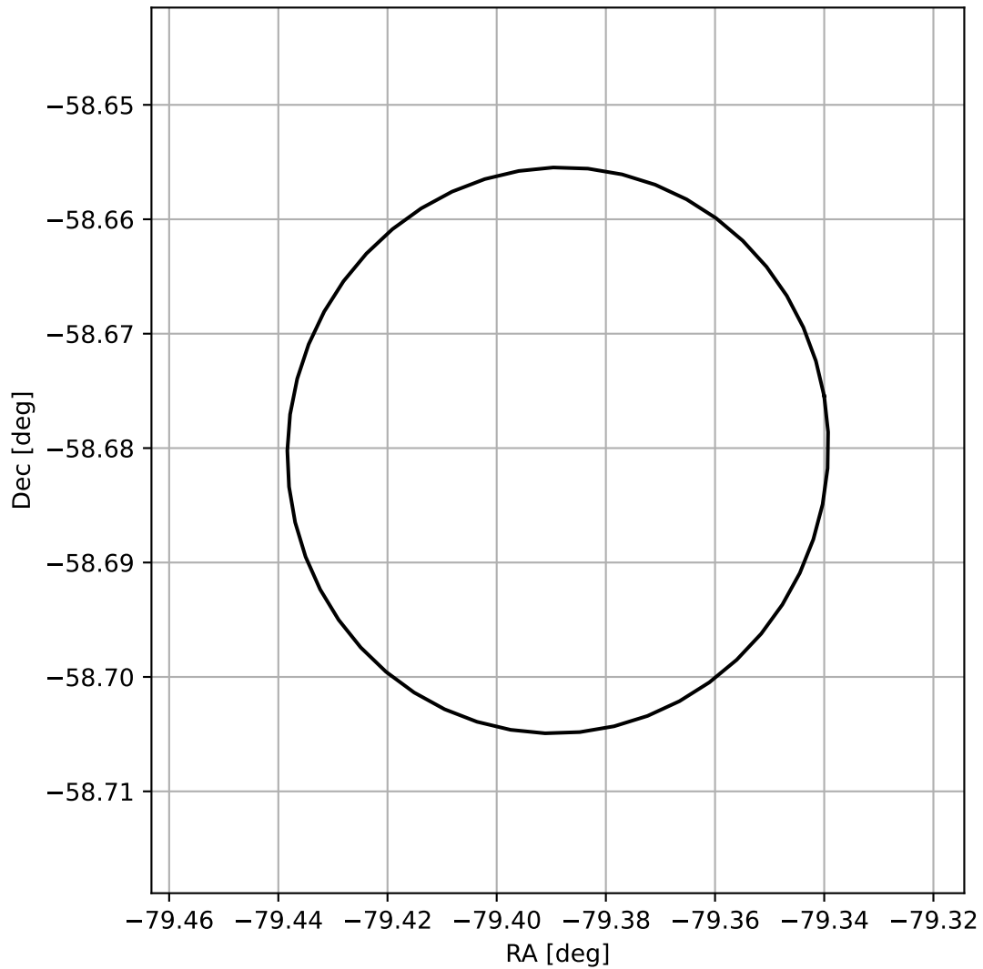
4FGL J1842.4-5840
