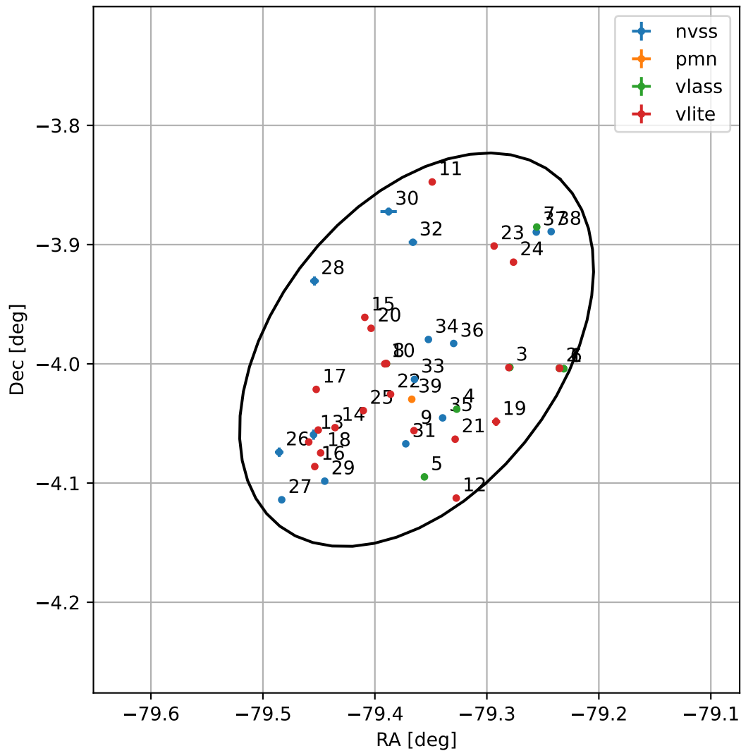
4FGL J1842.5-0359
