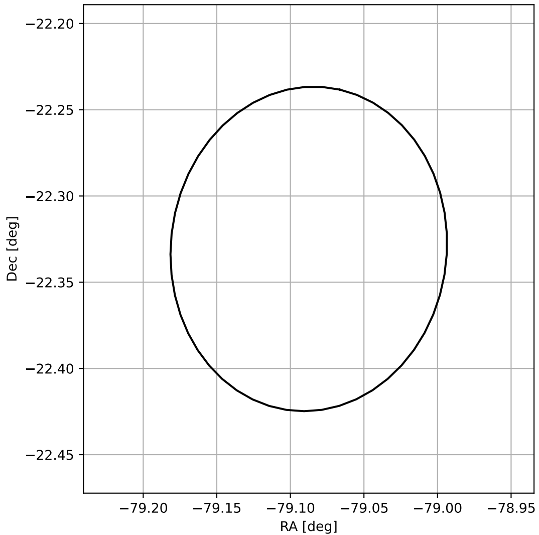
4FGL J1843.6-2219
