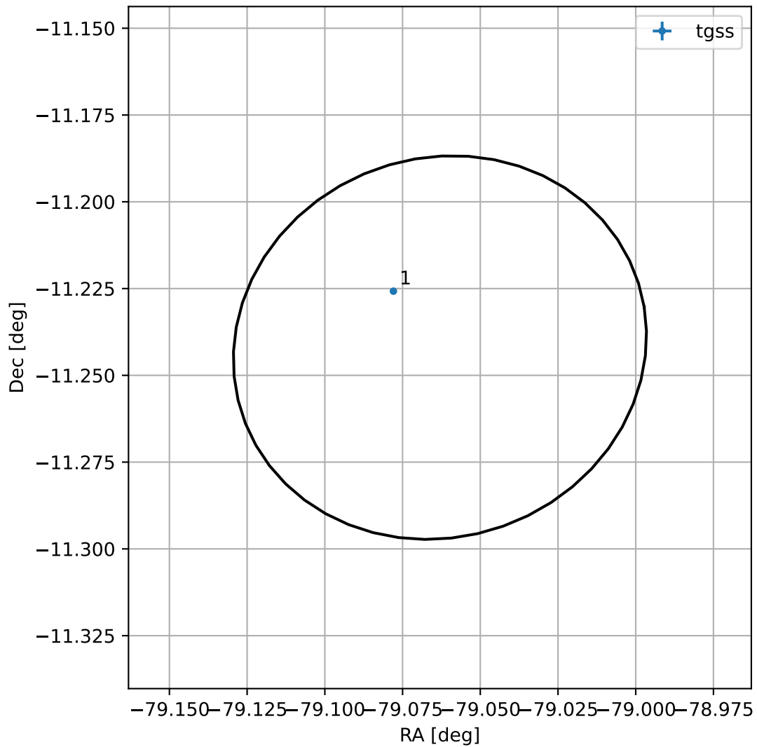
4FGL J1843.7-1114
