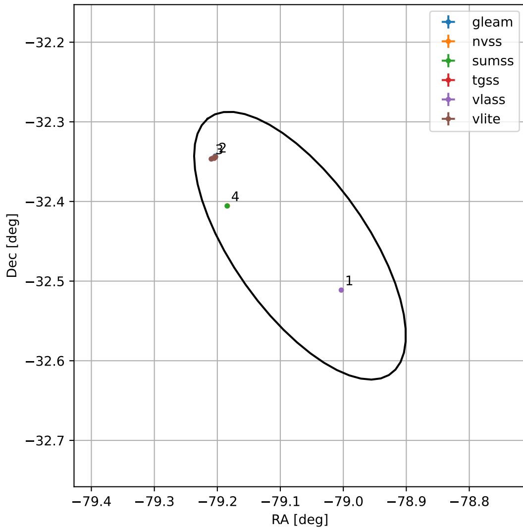
4FGL J1843.7-3227
