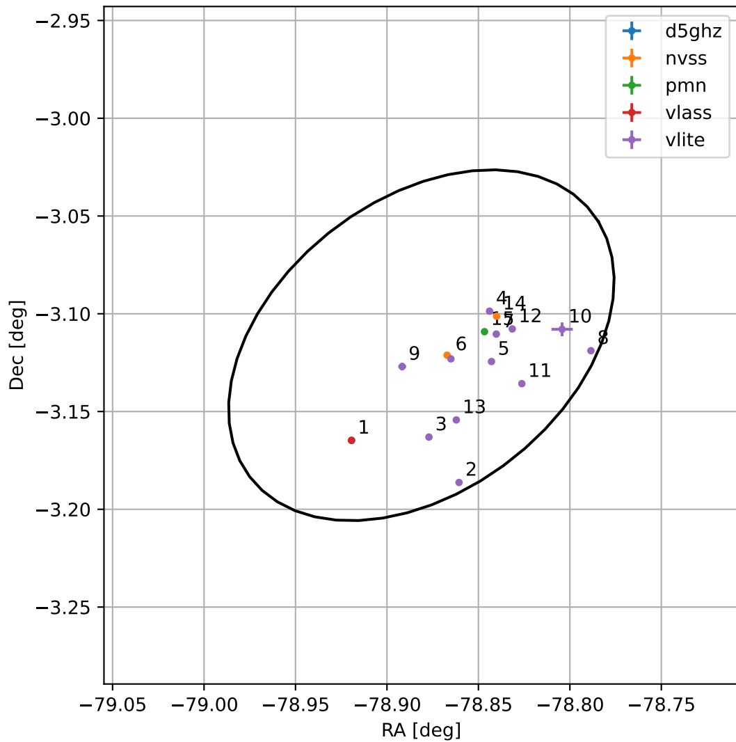
4FGL J1844.4-0306
