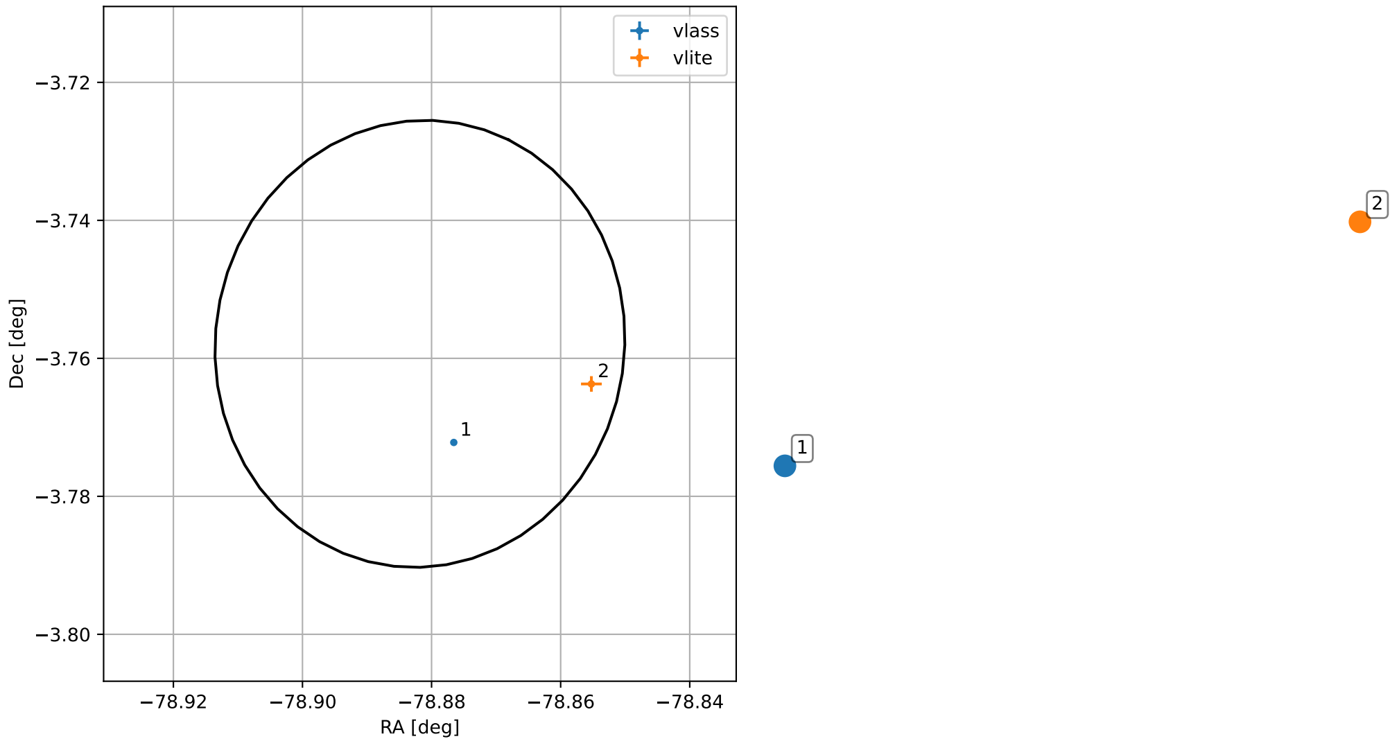
4FGL J1844.4-0345
