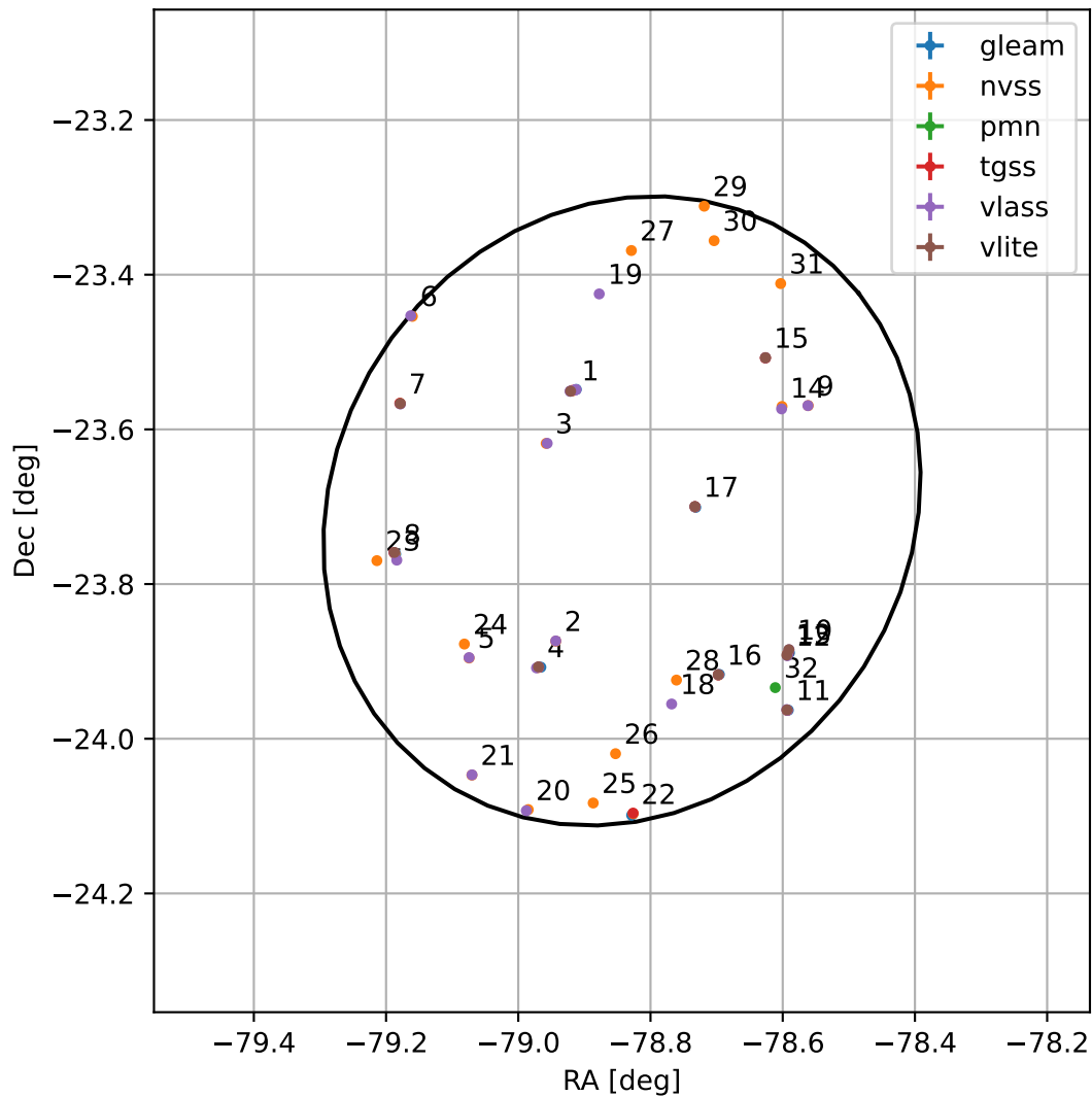
4FGL J1844.6-2342
