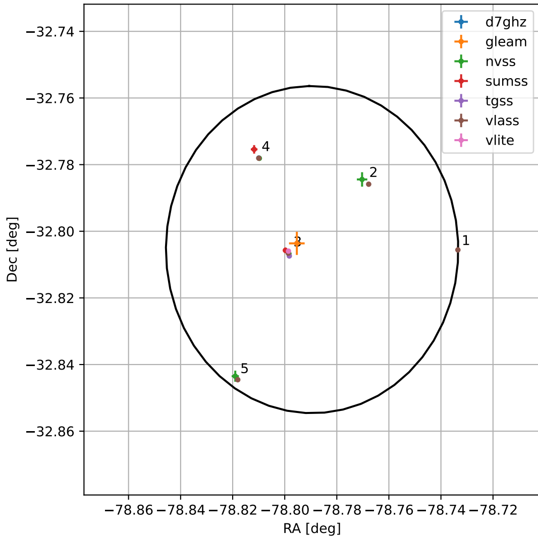
4FGL J1844.8-3248
