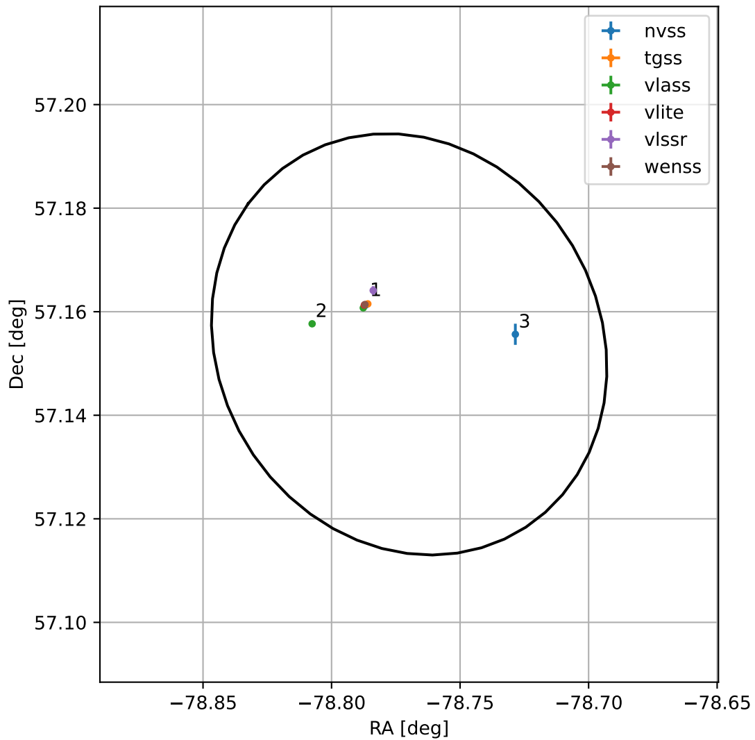
4FGL J1844.9+5709
