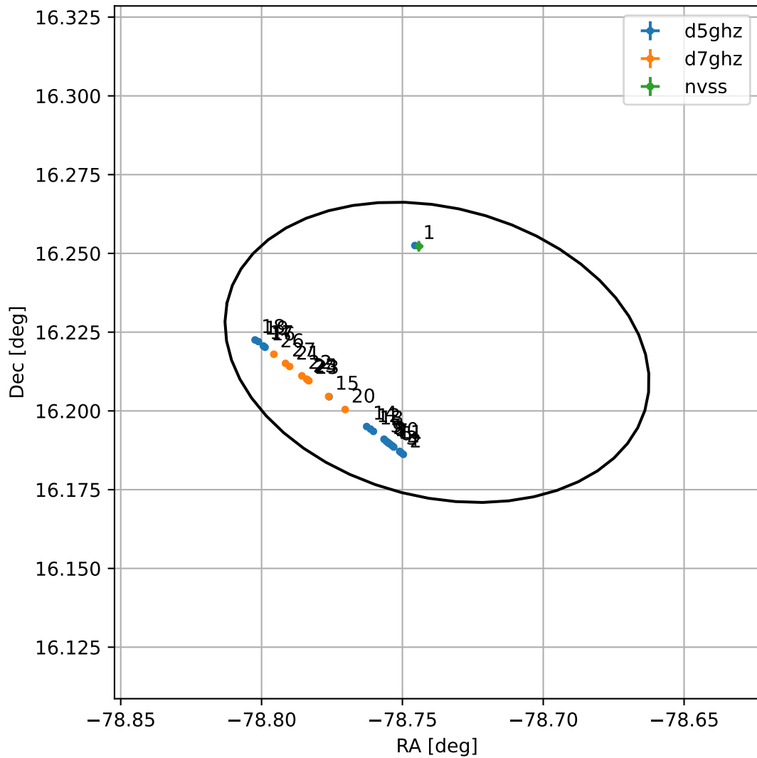
4FGL J1845.0+1613
