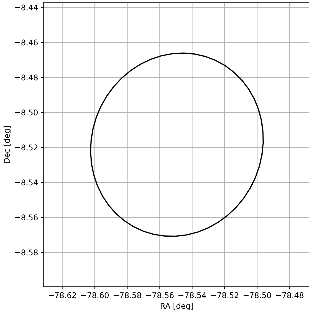
4FGL J1845.8-0831
