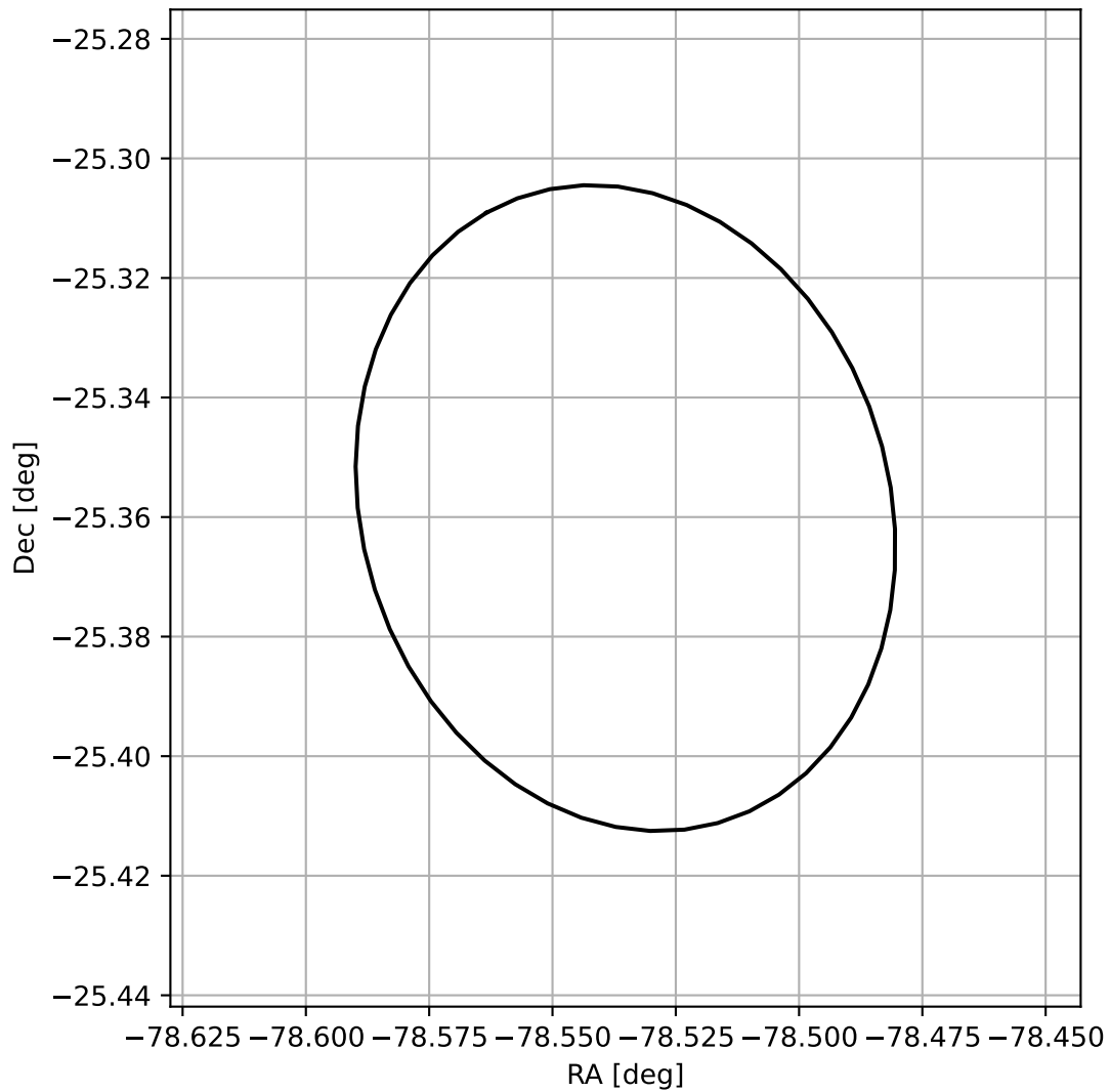
4FGL J1845.8-2521
