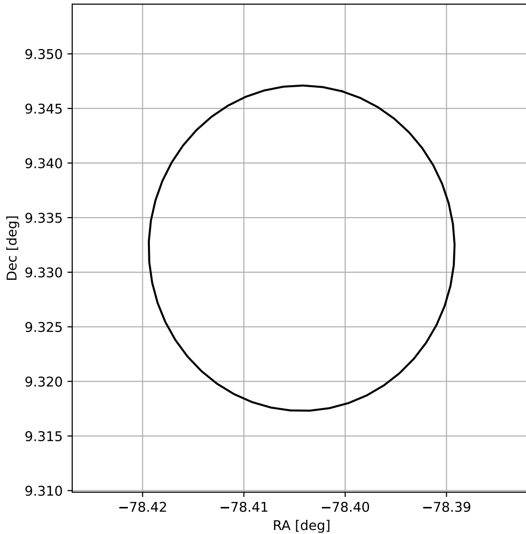
4FGL J1846.3+0919
