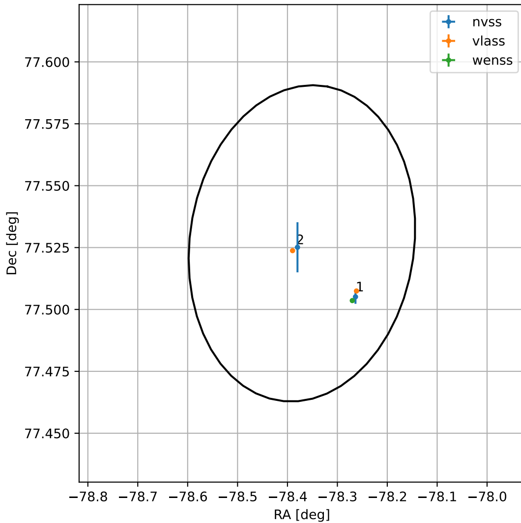
4FGL J1846.5+7731
