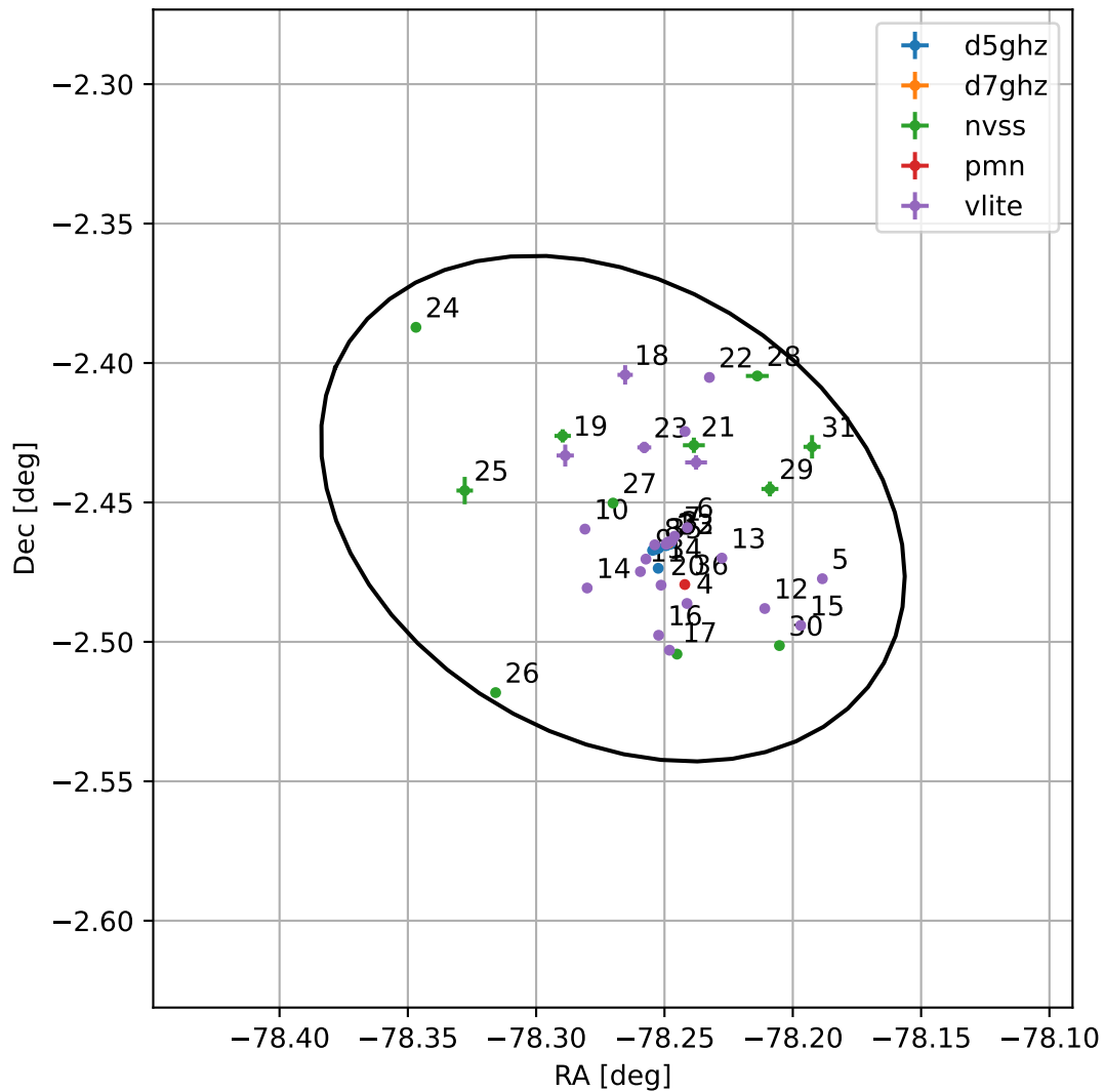
4FGL J1846.9-0227
