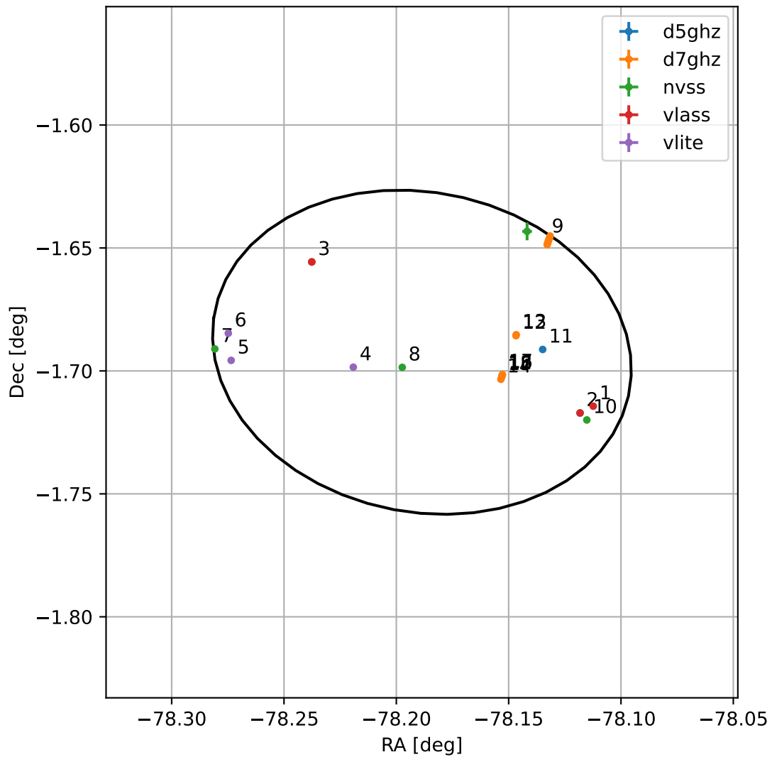
4FGL J1847.2-0141
