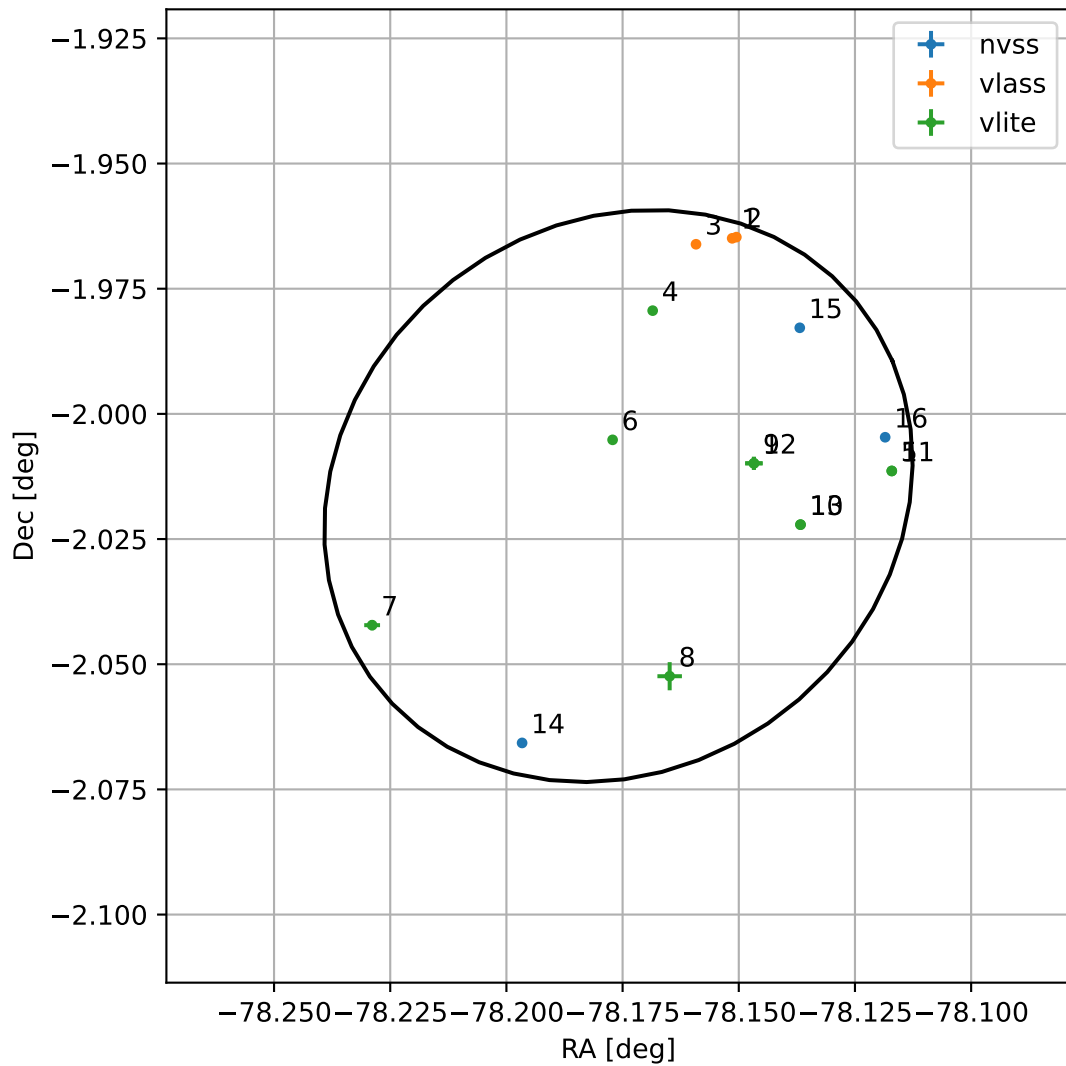
4FGL J1847.2-0200
