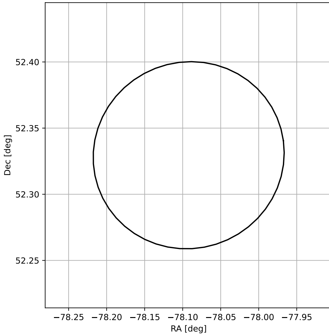
4FGL J1847.6+5219
