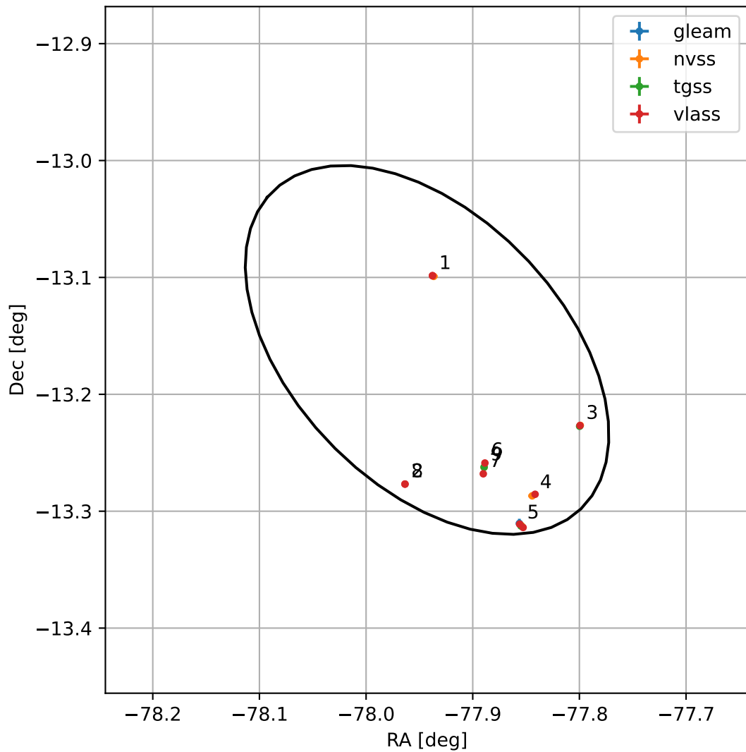
4FGL J1848.2-1309
