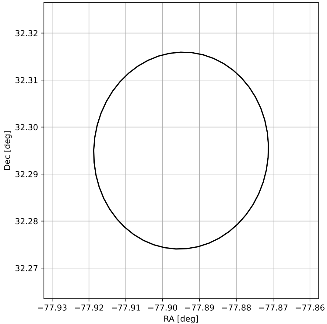
4FGL J1848.4+3217
