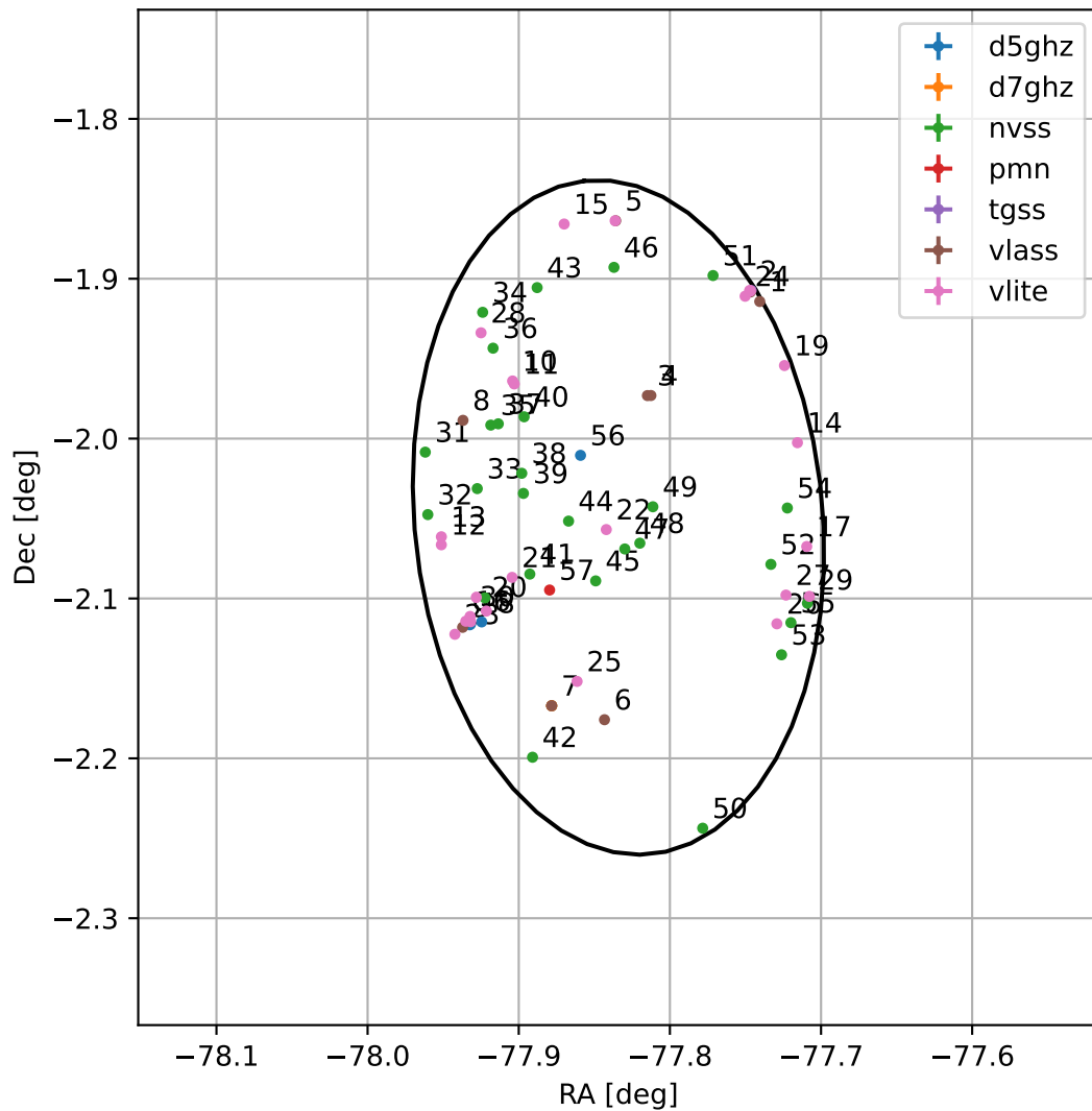
4FGL J1848.6-0202
