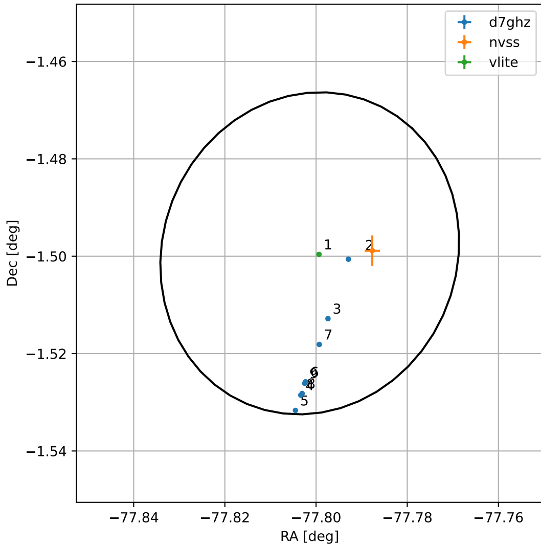
4FGL J1848.7-0129
