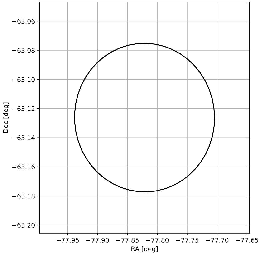
4FGL J1848.7-6307
