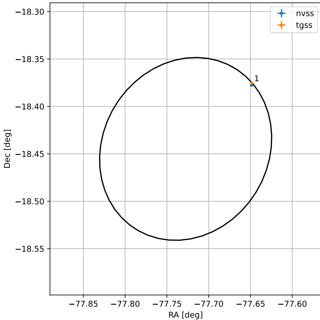
4FGL J1849.0-1826
