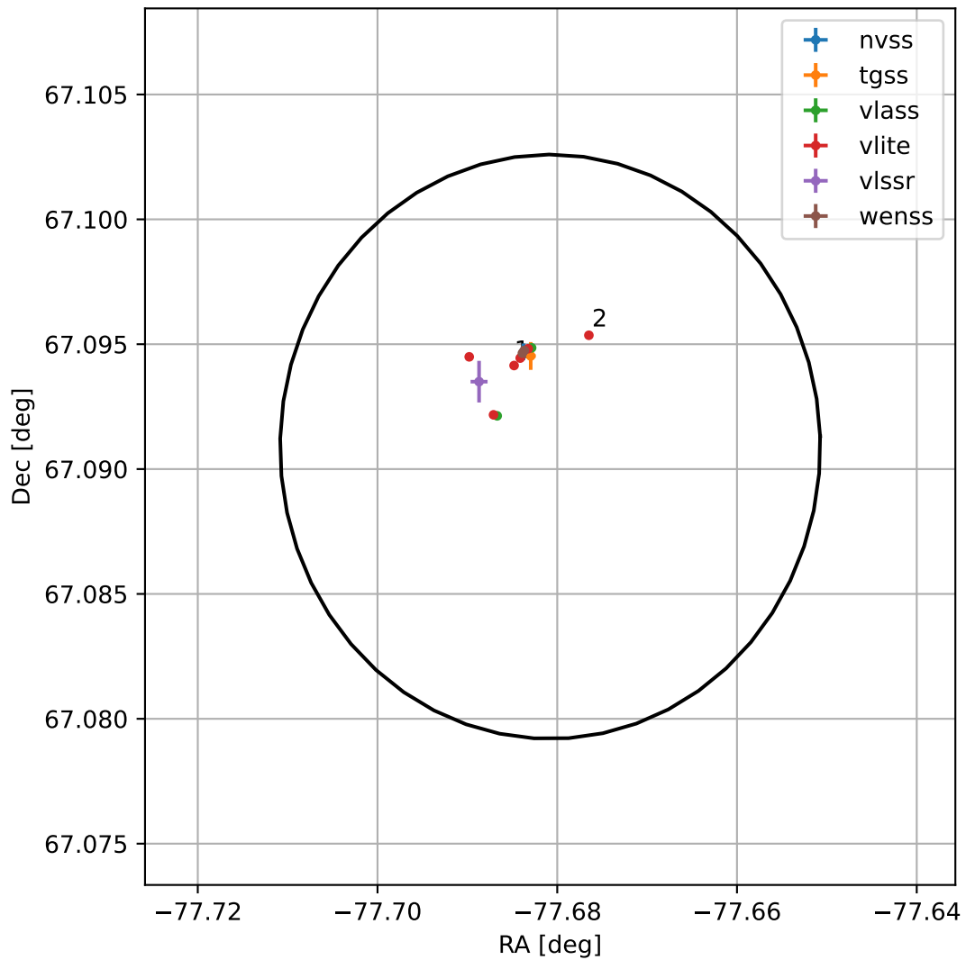
4FGL J1849.2+6705
