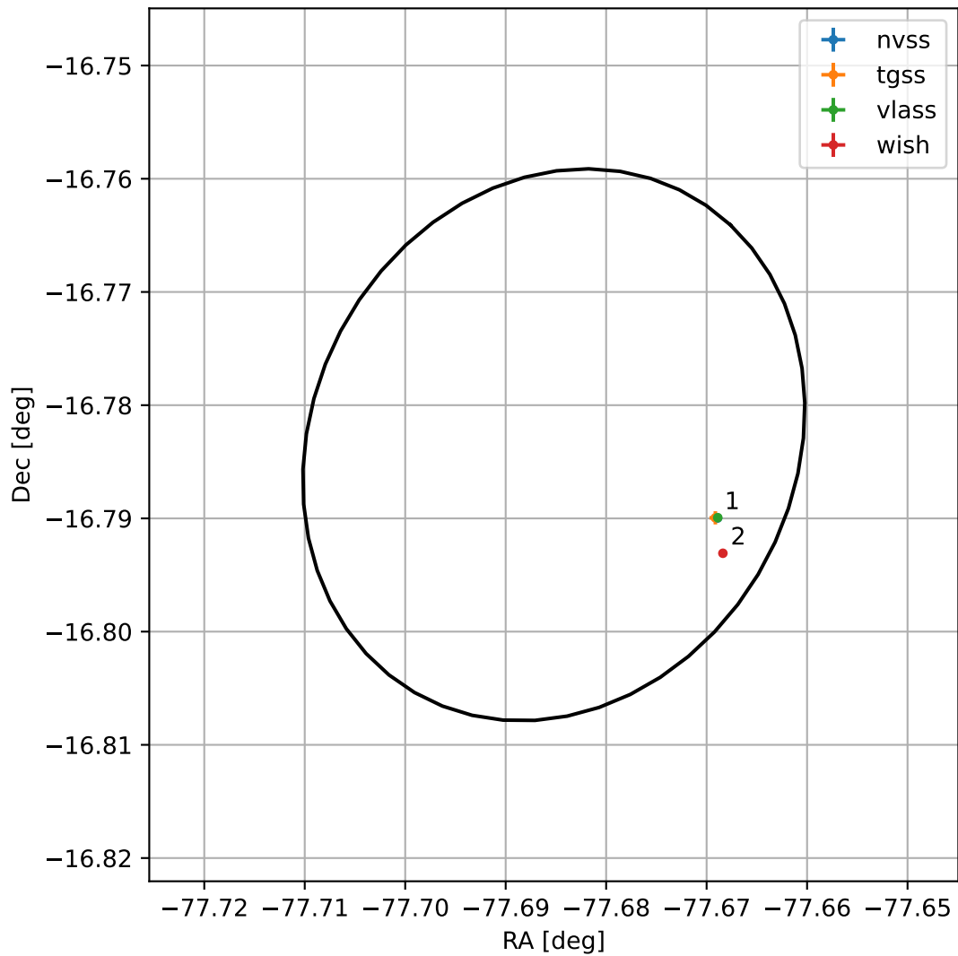
4FGL J1849.2-1647
