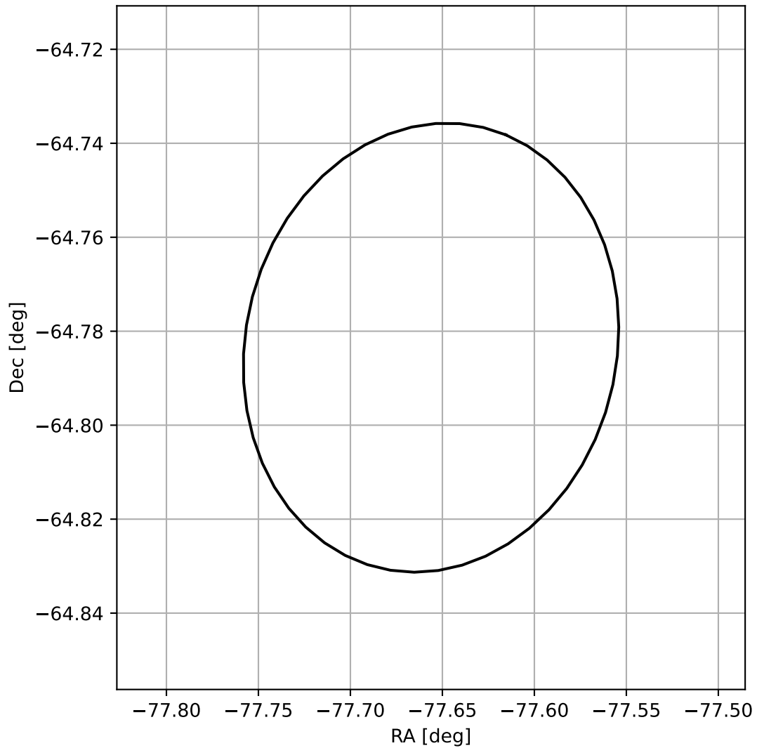
4FGL J1849.3-6447
