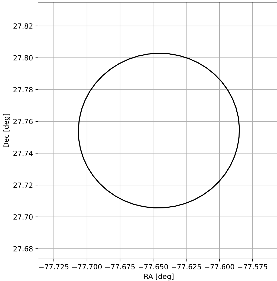
4FGL J1849.4+2745
