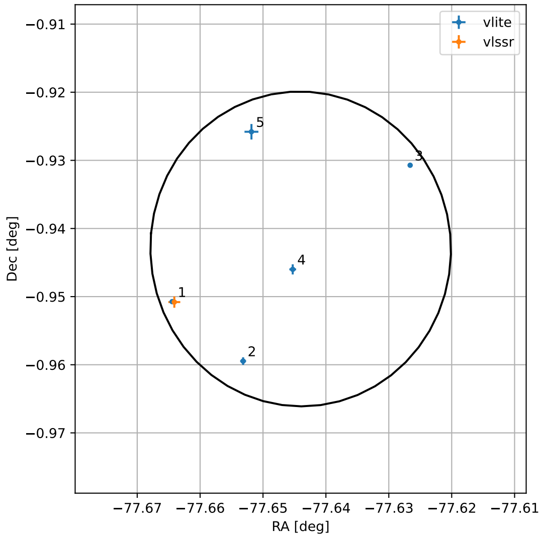
4FGL J1849.4-0056
