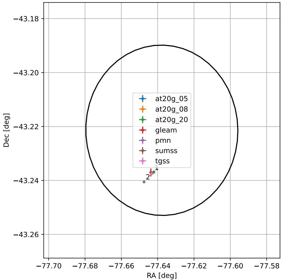
4FGL J1849.4-4313
