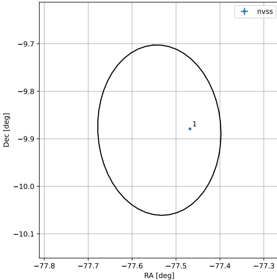
4FGL J1849.8-0952
