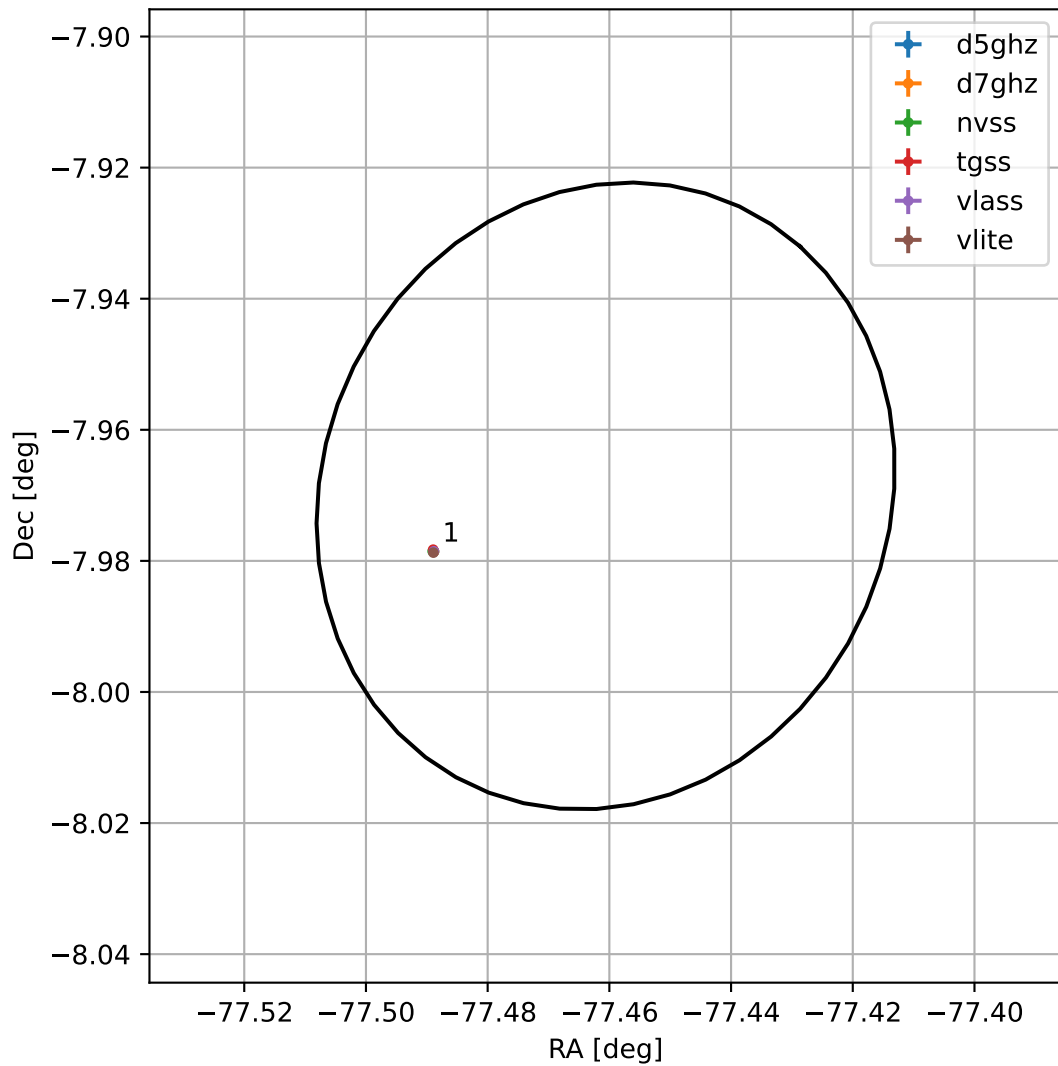
4FGL J1850.1-0758
