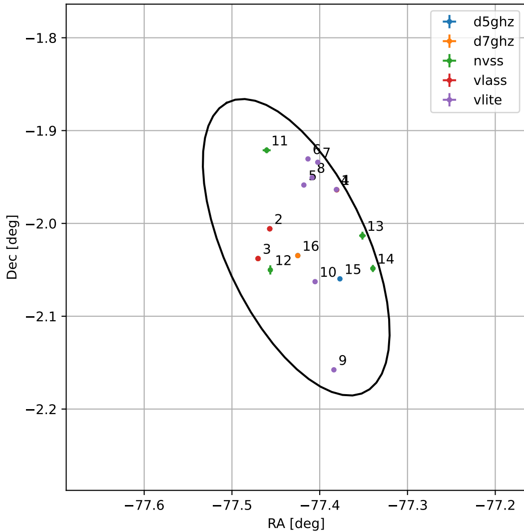
4FGL J1850.2-0201
