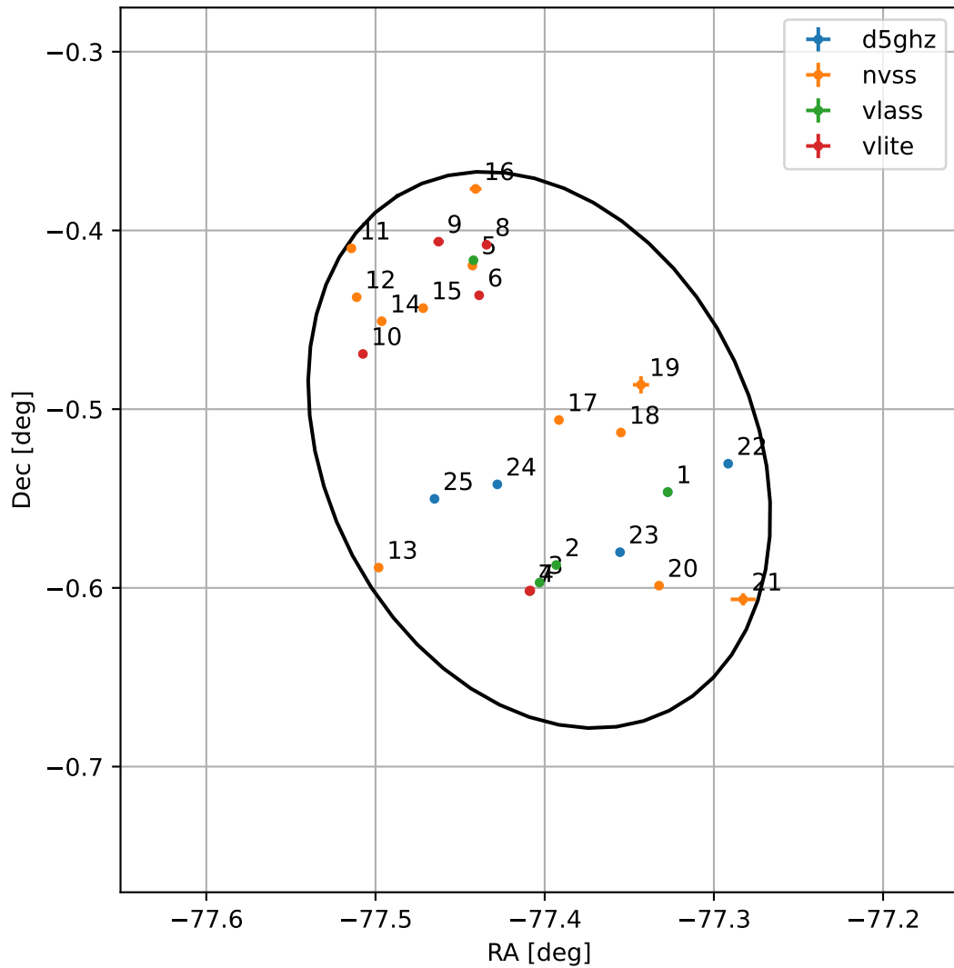
4FGL J1850.3-0031
