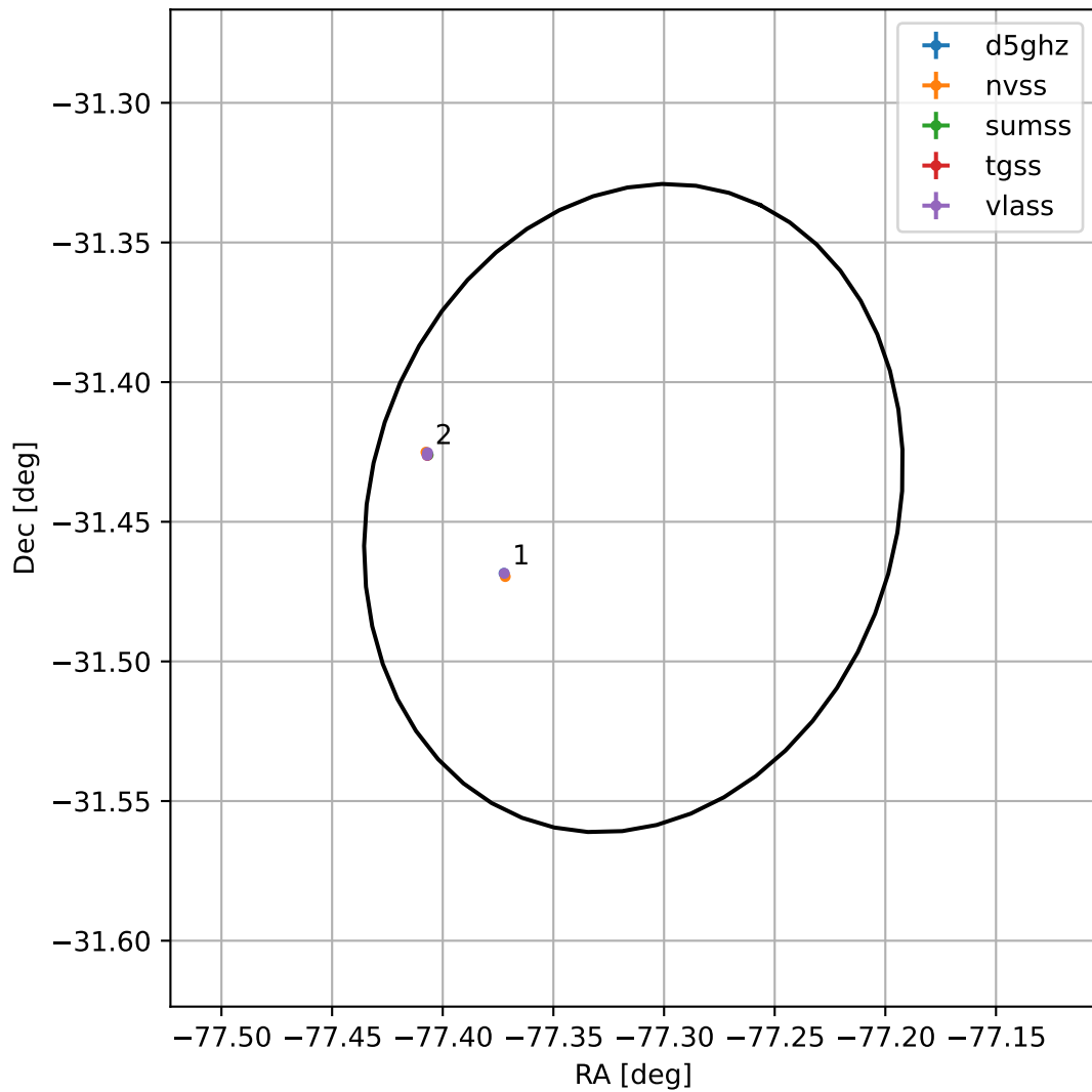
4FGL J1850.7-3126
