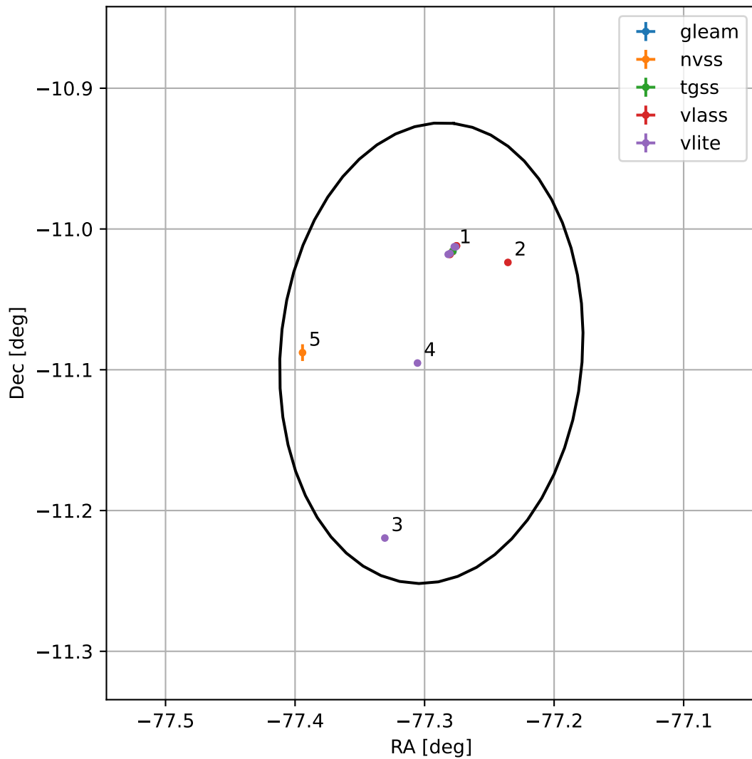
4FGL J1850.8-1105
