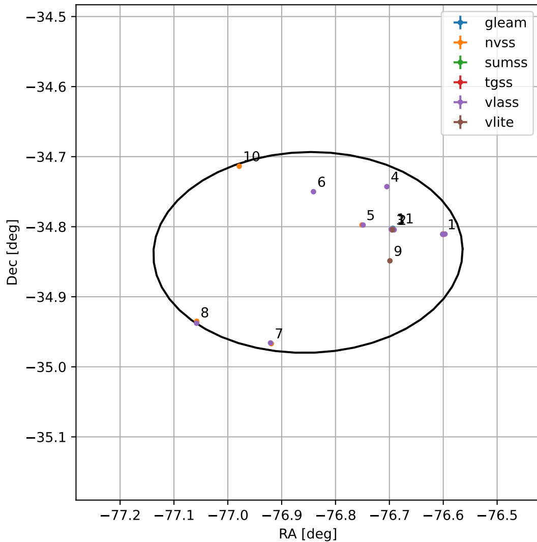
4FGL J1852.5-3450
