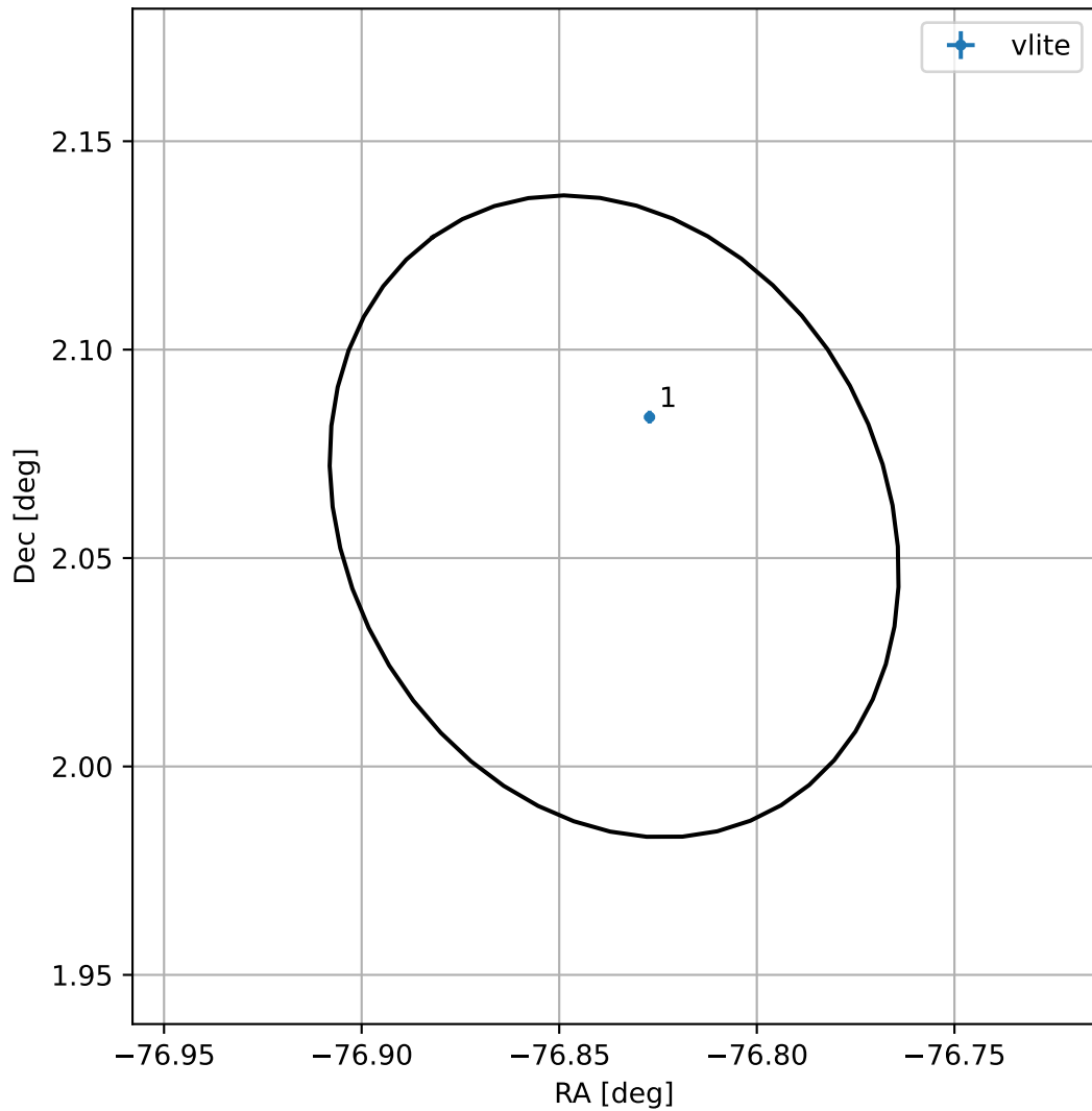
4FGL J1852.6+0203
