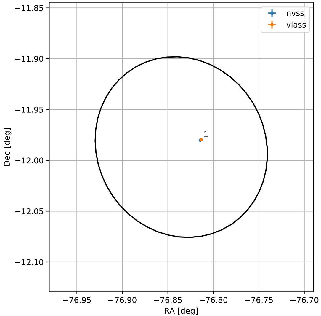
4FGL J1852.6-1159
